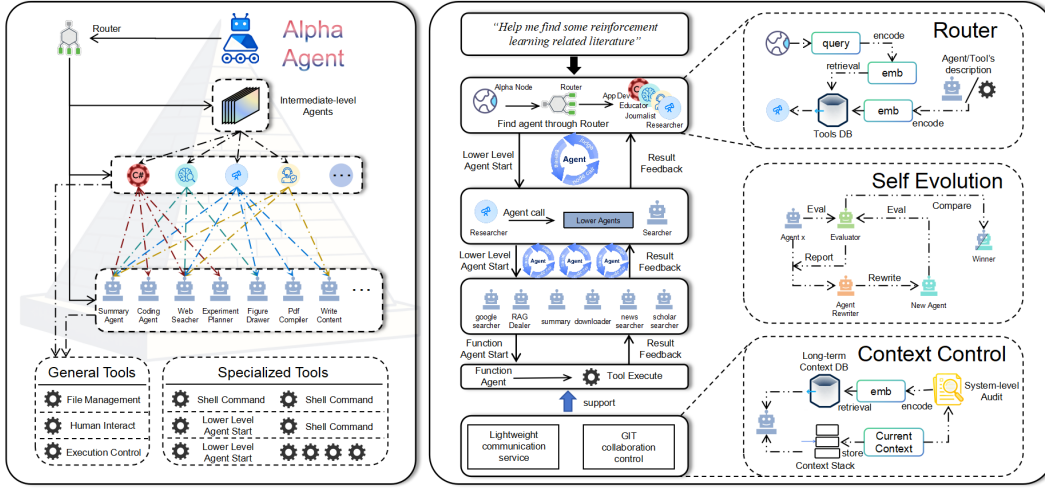
Figure 1: InfiAgent Framework Architecture. Left: An intuitive Pyramid-like agent organization architecture of InfiAgent, featuring a Router that redirects all user queries to avoid layer-by-layer tool search. Right: InfiAgent’s framework workflow schematic, highlighting three key modules: Router, Self Evolution, and Context Control.
