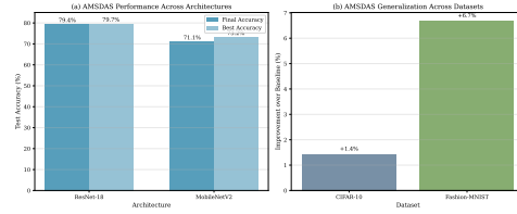
Figure 2: Architecture and dataset generalization analysis. (a) Comparison between ResNet-18 and MobileNetV2 shows consistent performance trends. (b) Cross-dataset evaluation demonstrates AMSDAS’s strong adaptation to different data distributions.
