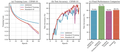
Figure 3: Training dynamics comparison between AMSDAS and baseline methods. (a) Training loss evolution shows AMSDAS maintains higher final loss, avoiding overfitting. (b) Test accuracy curves demonstrate AMSDAS’s superior stability. (c) Performance comparison across different datasets confirms the consistent benefits.
