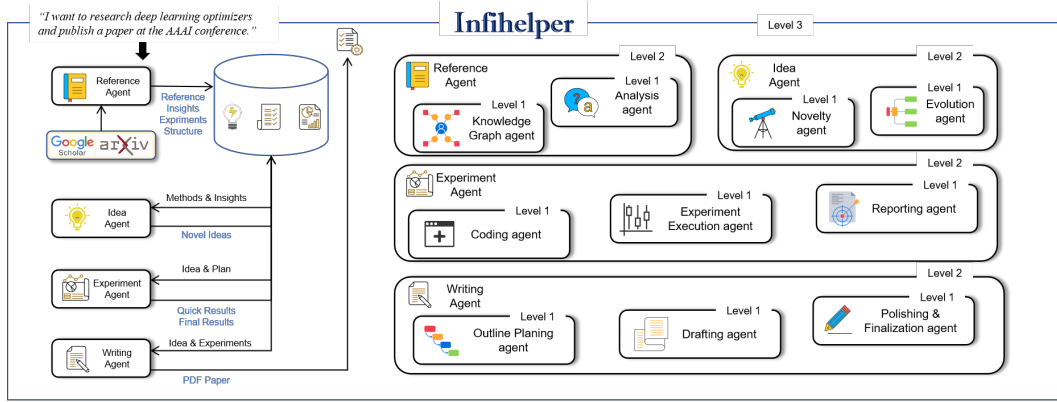
Figure 2: The Overall Structure of Our InfiHelper. This structure is initially generated autonomously by the InfiAgent Framework and then refined through human optimization. The lower-level agents serve as components of higher-level agents, which are not directly designed to operate within a fixed workflow. The workflow on the left side represents one of the potential operational workflows of the top-level agent, InfiHelper.
