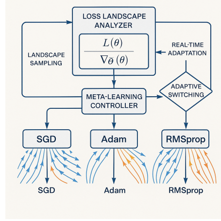
Figure 1: Architectural overview of the MetaOpt optimizer, showing the Loss Landscape Analyzer, Meta-Learning Controller, and Adaptive Switching components. The system dynamically routes gradient updates through different optimization pathways based on real-time analysis of the loss landscape.
