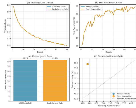
Figure 1: Detailed ablation analysis comparing full AMSDAS with early-layers-only configuration. (a) Training loss curves show near-identical optimization trajectories. (b) Test accuracy evolution demonstrates that early layer smoothing captures most performance benefits. (c) Convergence efficiency analysis confirms both configurations achieve 41.1% loss reduction rate. (d) Generalization gap scatter plot reveals similar training-test accuracy relationships.
