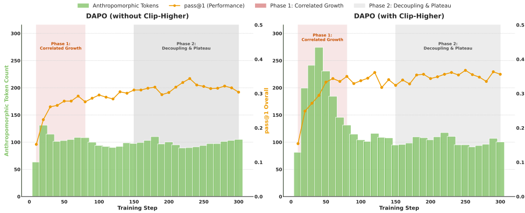
Figure 2: DAPO training dynamics on Qwen3-8B. Left: without Clip-Higher; Right: with Clip-Higher. In both settings we observe two phases—an early correlated growth between anthropomorphic token frequency and pass@1, followed by a decoupling then plateau . While Clip-Higher averts collapse, it does not prevent the later performance stall.
