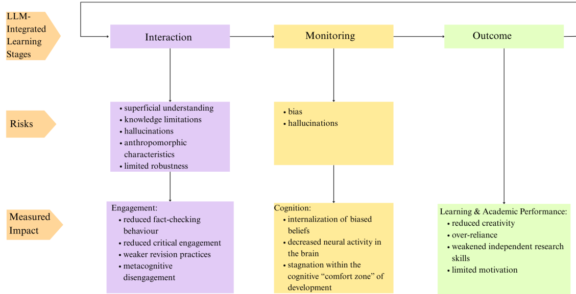
Fig. 6. LLM-Risk Adapted Learning Model (IMO), adapted from SRL theory, illustrating how risks emerge and compound across Interaction, Monitoring, and Outcome stages.
