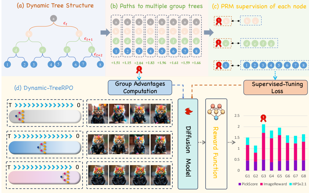
Figure 2: The framework of Dynamic-TreeRPO. (a) Dynamic Tree Structure. Noise intensity is dynamically introduced for the nodes of each layer in the tree structure. (b) Paths to multiple group trees. For each path, the highest reward score is selected. (c) PRM supervision of each node. The node with the maximum reward is used to supervise the model’s predictions at each layer. (d) Training procedure of Dynamic-TreeRPO.
