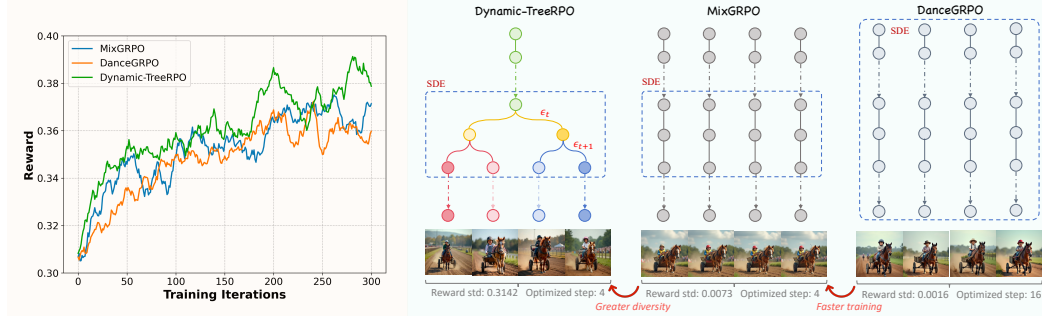
Figure 1: Compare with the previous method. Left : The reward curve during training shows that Dynamic-TreeRPO converges more rapidly than both DanceGRPO and MixGRPO, and ultimately achieves significantly better results than either of them. Right : Visualization of the different structures. Dynamic-TreeRPO employs a tree structure with a sliding window mechanism. MixGRPO utilizes a sliding window structure, where SDE is applied only during the sliding window period. In contrast, DanceGRPO applies SDE throughout the entire process.
