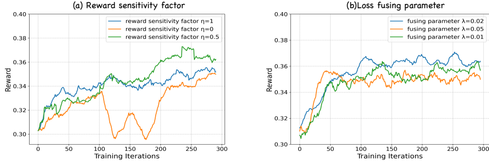
Figure 4: Ablation Studies on reward sensitivity factor and balancing parameter in LayerTuning-RL.
