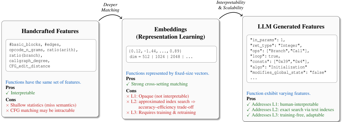
Figure 1: Evolution of features in BCSD. Left: Handcrafted statistics are interpretable, but shallow and sometimes intractable (CFG). Middle: Deep embeddings improve matching, but suffer from L1–L3 (interpretability, scalability–accuracy, training dependency). Right: Our LLM-generated structured features are interpretable, searchable via inverted/relational indexes, and training-free, addressing L1–L3, while improving practicality.
