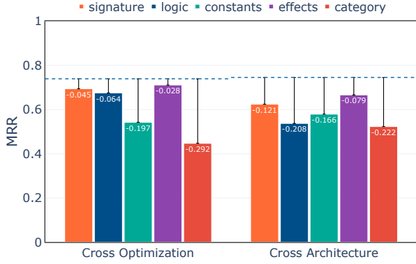
Figure 7: MRR with one prompt section removed using Gemini 2.5 Flash. Cross-optimization retrieval is between O0–O3 on x86–64, and cross-architecture retrieval is between ARM and x86–64 (at O2). Both use a pool of 100 functions. Dotted lines indicate MRR without section removal; smaller bars imply greater impact.
