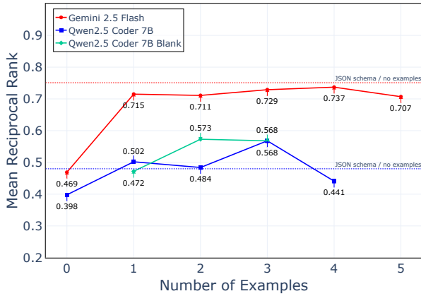
Figure 6: MRR for cross-optimization retrieval versus prompt examples. Functions are compiled for x86-64, using a pool of 100 functions. Retrieval is between 00-03 for Gemini 2.5 Flash and 00-01 for Qwen2.5 Coder 7B.
