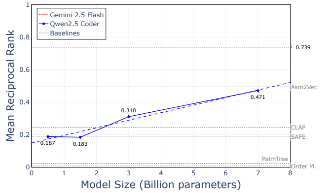
Figure 5: MRR for cross-optimization retrieval versus LLM parameters. All functions are compiled for ARM, with retrieval between O0–O1 using a pool of 1,000 functions. Prompts include three few-shot examples.
