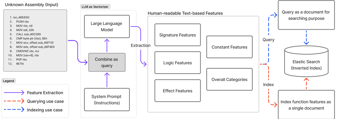
Figure 4: Workflow of our method in both the indexing and searching use cases.
