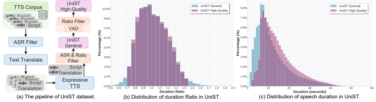
Figure 3: Overview of the UniST data construction pipeline and analysis of duration ratio and speech duration distributions.
