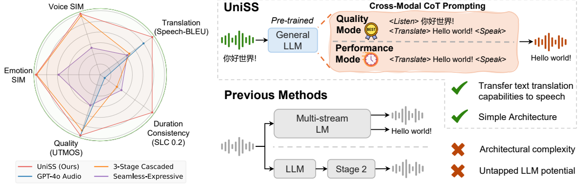
Figure 1: UniSS integrates pre-trained text LLMs and transfers their translation capabilities to the speech domain. UniSS outperforms both end-to-end S2ST systems and cascaded systems on translation fidelity, voice preservation, duration consistency, and speech quality.
