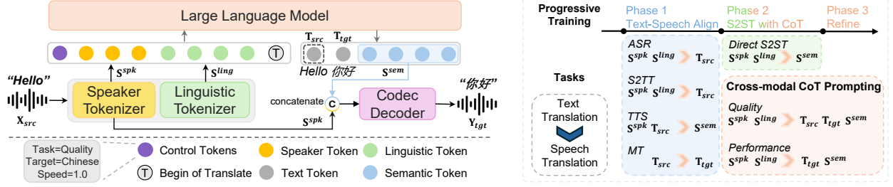
Figure 2: Overview of UniSS, cross-modal CoT prompting, and 3-phase progressive training. Control Tokens instruct the task (S2ST Quality Mode in the figure), target language (Chinese in the figure), and output speed ratio compared with input (usually 1.0 means 1:1 duration matching).
