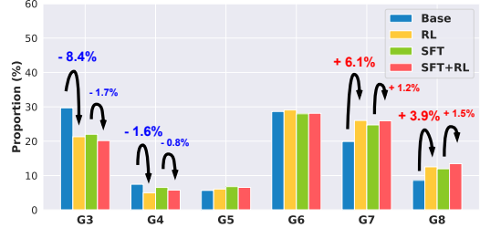
Figure 9: Proportion of Graphlets. Bar graph shows results averaged across all models in Table 1 and datasets, AIME24, AIME25, and AMC23. Arrows indicate the change in graphlet proportion after RL. See Section C.2 for results by model and dataset.
