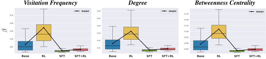
Figure 5: Exponential Decay Rate for Visitation Frequency, Degree, Betweenness Centrality. Box plots show the estimated exponential decay rate \beta across all problems in AIME24, AIME25, and AMC23 for the 1.5B models in Table 1. See Figure 23 for complete results.
