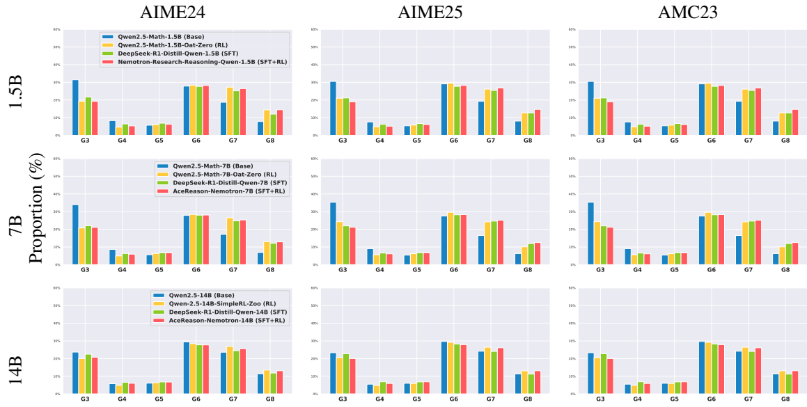
Figure 26: Proportion of 4-node Graphlets. Graphlet proportions for models in Table 1 on AIME24, AIME25, and AMC23.
