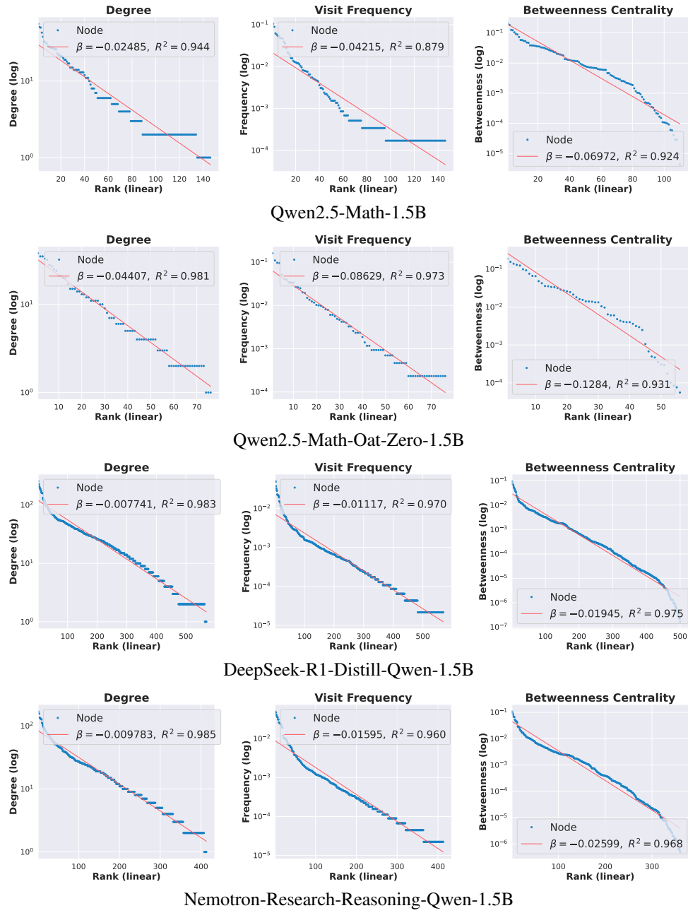
Figure 22: Example of Exponential Decay Rate Estimation. Linear regression on a semi-log plot of degree, visitation frequency, and betweenness centrality in AIME24 Problem #1.
