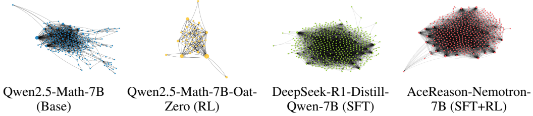
Figure 19: Visualization of Reasoning Graphs. Results of 7B models in Table 1 on AIME24 Problem #1. Node encodes the node occurrence count, and edge length has no meaning. Graphs are visualized using Kamada-Kawai layout in NetworkX.
