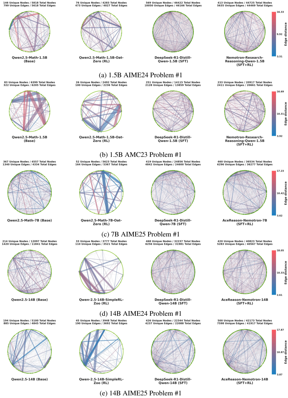
Figure 20: Reasoning Graphs Examples. Nodes arranged sequentially on circle, consistent across examples. Edge thickness encodes transition frequency, and edge color encodes edge distance.
