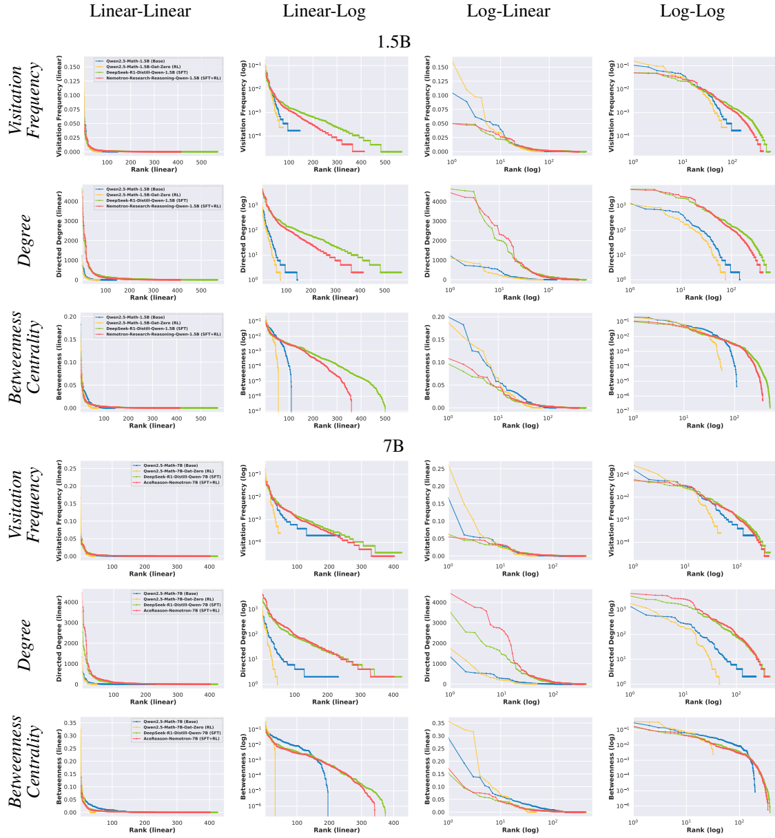
Figure 21: Rank plots for Visitation Frequency, Degree, and Betweenness Centrality. Results for 1.5B (top) and 7B (bottom) models in Table 1 on AIME24 Problem #1.
