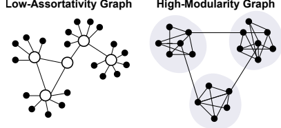
Figure 6: Illustration of the Low-Assortativity Graph (Left) and High-Modularity Graph (Right).
