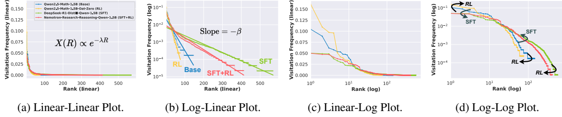
Figure 4: Visitation Frequency Rank Plot. Results from the 1.5B model in Table 1 on AIME24 Problem #1, shown with four combinations of linear/log scales on the x- and y-axes. The rank plot approximately follows an exponential law, showing near-linear behavior on a log-linear scale. See Figure 21 for more examples.
