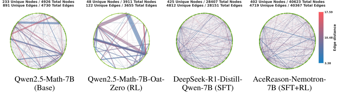
Figure 3: Reasoning Graph Example. Directed reasoning graph for AIME24 Problem #1 built from 256 responses across the 7B models in Table 1. Nodes are arranged sequentially on a circle, consistent across examples. Edge thickness encodes transition frequency, and edge color encodes edge distance. For more examples, please refer to Figure 19 and Figure 20.
