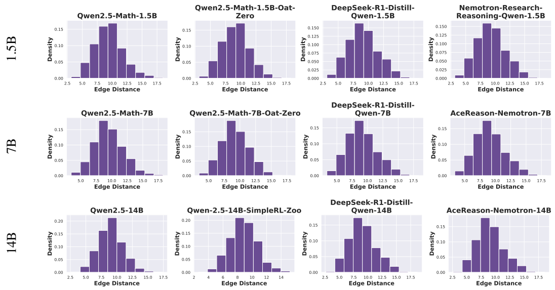
Figure 24: Edge Distance Distribution. Frequency distribution of edge distances shown in bins across models in Table 1 and datasets, AIME24, AIME25, AMC23.
