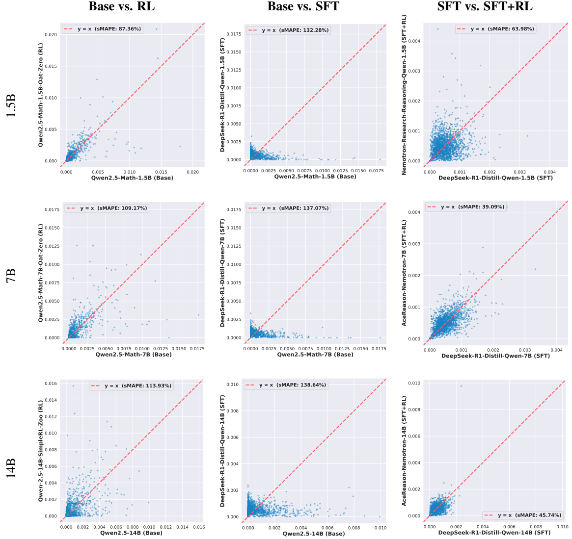
Figure 25: Visitation Frequency Scatter Plot Between Two Models. Each plot represents a node, with coordinates indicating the visitation frequency in the integrated graph across all AIME24 problems for two models in Table 1. The closer the plots are to the line y = x , the more similar their visitation frequency of that node between two models.
