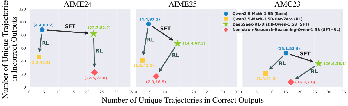
Figure 2: Effect of RL and SFT on the Number of Unique Trajectories. The x-axis represents the number of correct clusters and the y-axis represents the number of incorrect clusters for trajectories before and after training of 1.5B models in Table 1. See Section B.3 for complete results and for additional results Section B.4.
