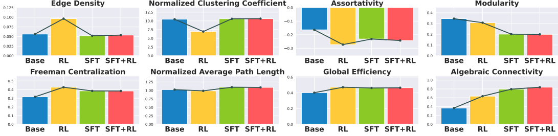
Figure 7: Comparison of eight graph metrics across Base, RL, SFT, and SFT+RL models. Values are averaged across different model sizes in Table 1 and three datasets, AIME24, AIME25, and AMC23. See Figure 27 for results by model size.
