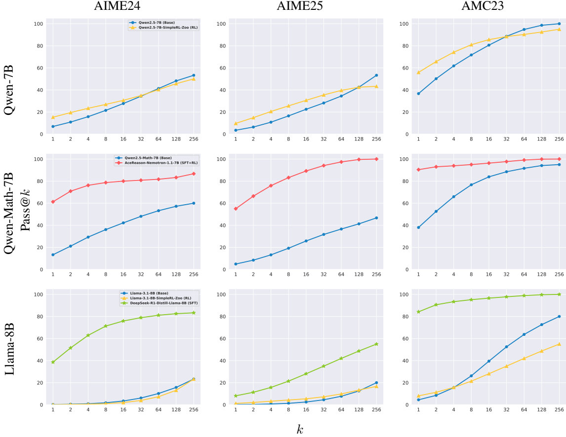
Figure 15: \text{Pass}@k performance curves for additional models. Models are from Table 2 that are not included in Table 1 and datasets are AIME24, AIME25, and AMC23.
