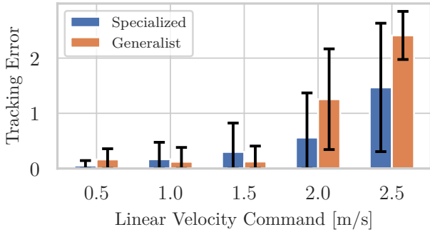
Fig. 8: Mean tracking error along multiterrain course for varying speed demands.
