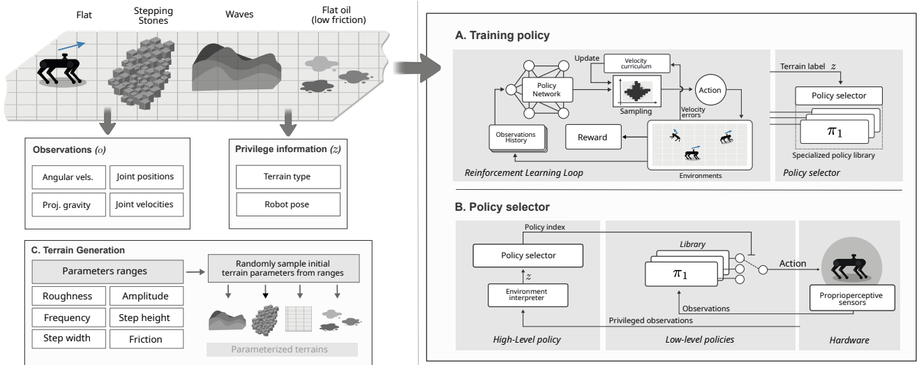
Fig. 2: System overview. (A) Training Policy : An RL policy receives a short history of proprioceptive observations, the previous action, and the commanded velocities. The reward blends command-tracking terms with penalties for high kinematic jerk and unstable contacts. A discrete curriculum grid over (v_x^{\text{cmd}}, \omega_z^{\text{cmd}}) is sampled; when a cell’s error \|v^{\text{cmd}} - v^{\text{base}}\| < \epsilon , its neighbors unlock, increasing difficulty. Trained policies are appended to a specialized policy library, each stored with its associated privileged observation z . (B) Policy Selector : A deterministic mapper parses the privileged vector z to extract the relevant cues and directly outputs the index i of the policy to run in the library; the selected \pi_i is applied until a new selection is triggered. (C) Terrain Generation : A parametric generator procedurally varies geometric and frictional properties to synthesize a set of challenging terrains.
