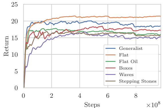
Fig. 4: Training curves of average return against simulation steps: generalist vs. five specialized policies.
