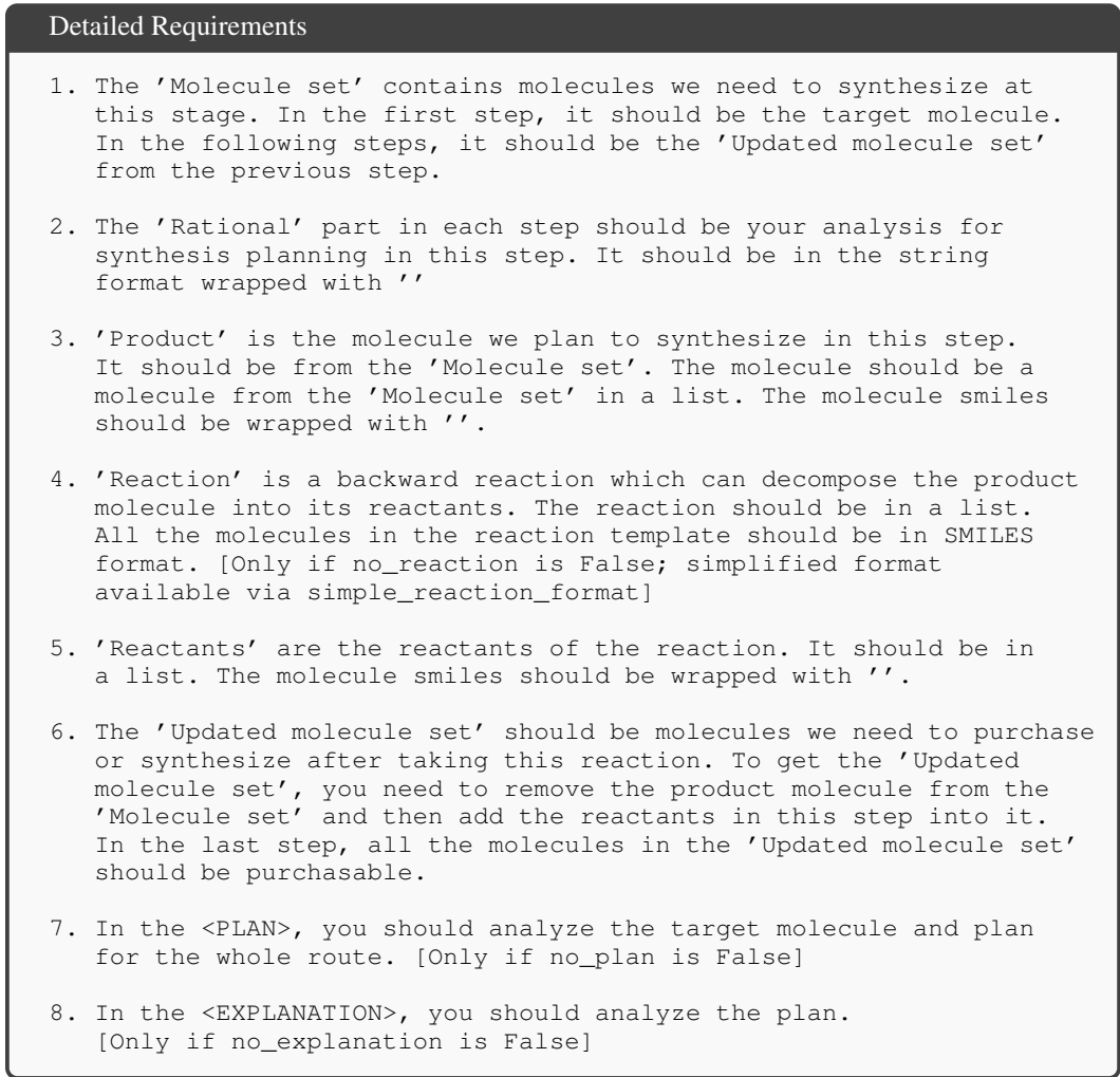
Figure 10: Detailed requirements section dynamically constructed based on ablation flags. Requirements are numbered sequentially with conditional inclusion.
