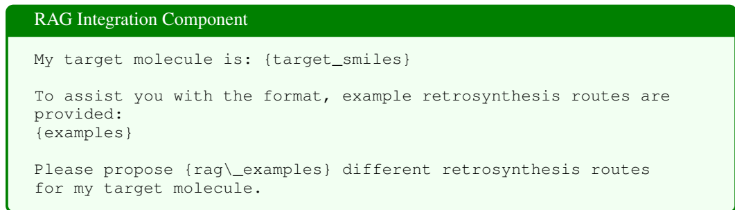
Figure 6: RAG integration with retrieved examples.
