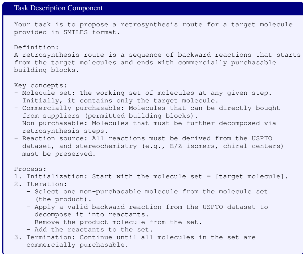
Figure 5: Task description component.
