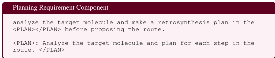
Figure 7: Planning requirement component.
