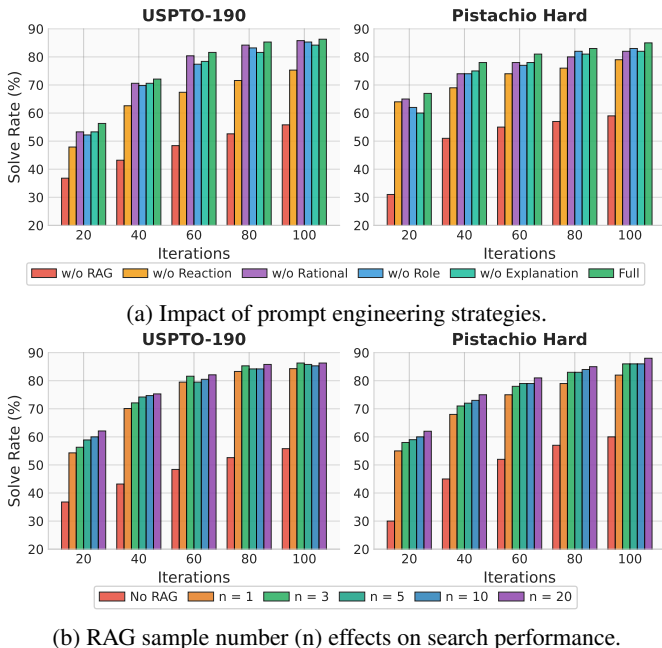
Figure 2: Component analysis on Pistachio Hard, USPTO-190.
