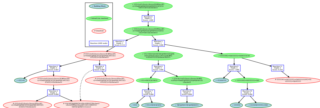
Figure 14: CCCc1c(Cc2ccc(-c3ccccc3C#N)cc2F)c(=O)n([C@H]2CC[C@H](OCC3(C(C)=O)CCC3)CC2)c2ncnn12 , USPTO-190, Visualization of AOT* search tree.
