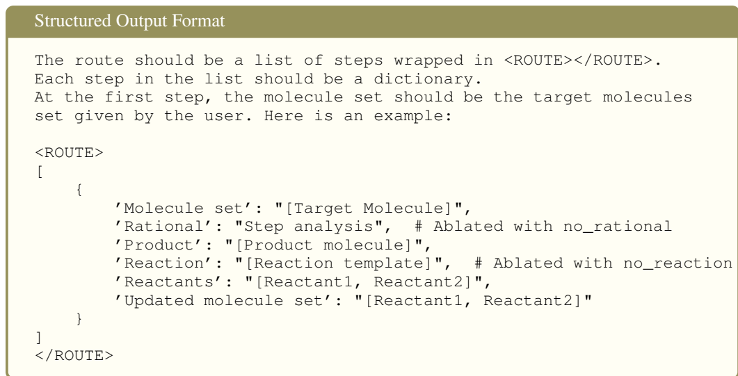
Figure 9: Structured output format.
