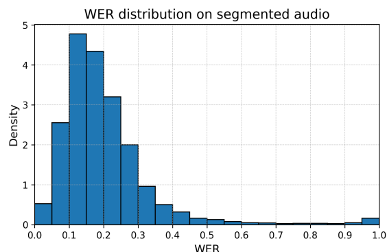
Figure 4: Distribution of WER values on segmented audio
