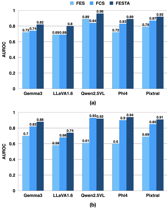
Figure 4: AUROC for uncertainty based on FES, FCS and FESTA on (a) BLINK, (b) VSR data.
