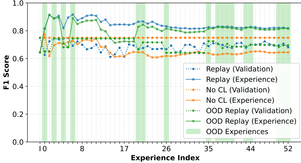
Figure 4: Continual learning performance over 53 sequential experiences comparing three deployment strategies: static baseline (No CL), continuous adaptation (Replay), and OOD-triggered selective adaptation (OOD Replay). Green regions indicate OOD detection triggers and the I standing for the initial performance.
