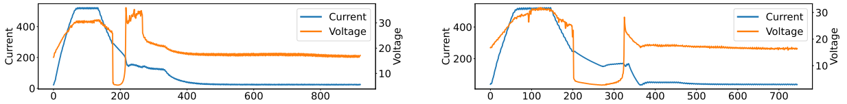
Figure 2: Representative current and voltage patterns from single welding cycles for overlap (left) and T-joint (right) configurations.
