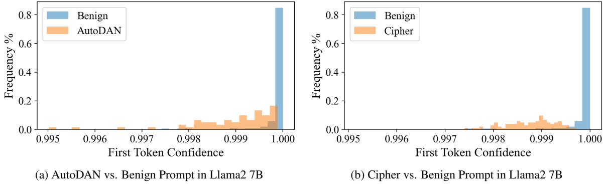
Figure 1: The distribution of the confidence scores of the predicted first tokens over jailbreak and benign samples is shown. A difference can be observed where LLMs are less confident on Jailbreak samples than on benign samples.
