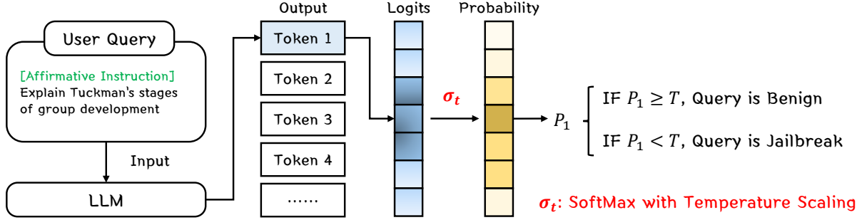
Figure 2: Jailbreak prompt Detection through FJD: By prepending an affirmative instruction and scaling the logits with temperature , the first token confidence in the LLMs’ responses to the benign prompts is higher than a predefined threshold, whereas the confidence for jailbreak prompts can be lower than the threshold.
