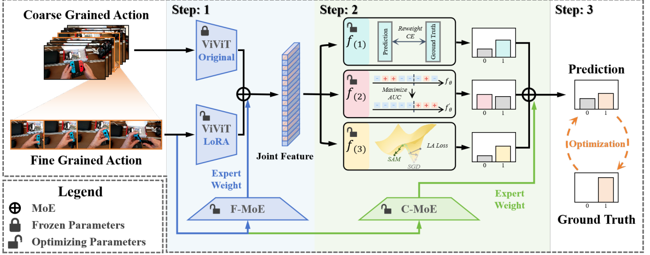
Figure 1. An overview of our DR-MoE method. Our method consists of two main stages. The first stage performs feature extraction by combining a frozen ViViT backbone and a LoRA-tuned ViViT backbone through a Feature Mixture-of-Experts (F-MoE) module. The second stage carries out classification by integrating the outputs of three independently trained classifiers using a Classification Mixture-of-Experts (C-MoE) module to generate the final prediction.
