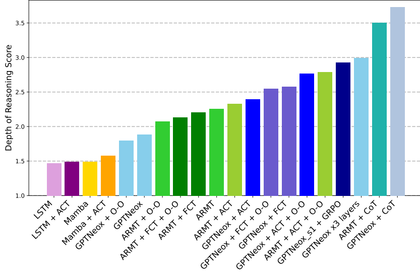
Figure 8: With GRPO as well as with ACT and Orbit-Orbit training depth of reasoning can be significantly extended. Average DepthScore = 1 + \sum_{i=2}^4 acc(i) , where acc(i) is the accuracy of predicting the (10 + i) th state based on the first 10 states.
