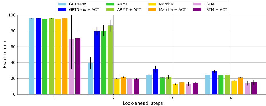
Figure 4: ACT significantly improves computational abilities of transformer-based models in multi-step prediction. Exact match of the x^{(T+k)} state prediction for look-ahead steps k \in \{1, 2, 3, 4\} for O-S training objective. Different models are shown in different colors.
