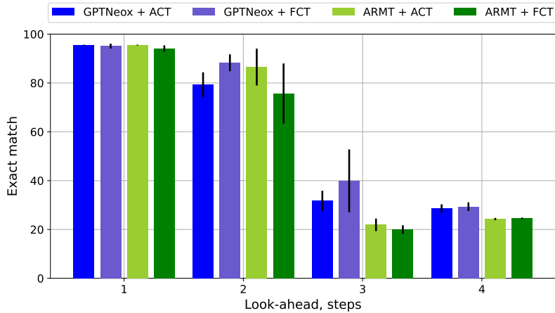
Figure 10: Fixed Computation Time (FCT) with 3 iteration steps performs on par with Adaptive Computation Time (ACT) in Orbit-State task. Exact match accuracy (mean \pm std) for cellular automata state prediction across different look-ahead horizons.
