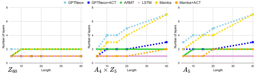
Figure 7: ACT significantly reduces the required models’ depth for the majority of group multiplication tasks. Each chart contains the information about the minimal required number of layers for solving task of given length with 70% exact match accuracy. GPTNeox and Mamba being TC^0 -limited models require more layers for solving deeper (longer in this case) tasks, while ARMT and LSTM solve them with constant number of layers.
