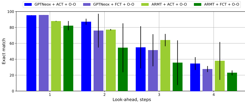
Figure 11: Fixed Computation Time (FCT) with 3 iteration steps underperforms Adaptive Computation Time (ACT) in Orbit-Orbit task. Exact match accuracy (mean \pm std) for cellular automata state prediction across different look-ahead horizons.
