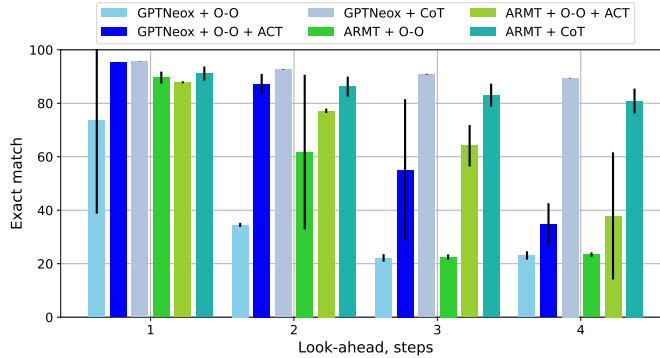
Figure 6: With step-by-step supervision, the CoT approach significantly outperforms the in-depth approach of ACT. While the performance of the depth-based methods decreases with the increasing look-ahead steps, breadth-based CoT succeeds in predicting up to all 4 steps. However, among the models without autoregressive generation, GPTNeox and ARMT with both ACT and O-O supervision perform the best.
