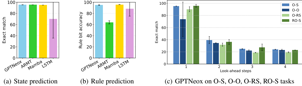
Figure 2: Single-step accuracy is near-perfect across models, but multi-step performance collapses. (a) Exact-match accuracy for single-step state prediction (O-S): all models except LSTM achieve >95\% . (b) Bit-wise accuracy for rule inference (O-RS): most architectures recover the hidden Boolean rule, yet ARMT trails the rest. (c) GPTNeox accuracy on variable-horizon prediction across the four task variants (O-S, O-O, O-RS, RO-S): accuracy falls steeply with look-ahead k .
