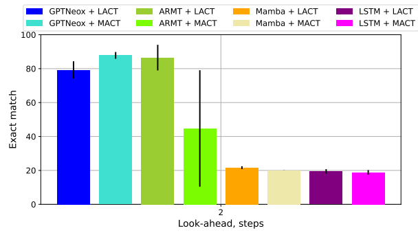
Figure 12: Layer-ACT performs similar or better compared to Model-ACT. Exact match on cellular automata state prediction task with look ahead 2.
