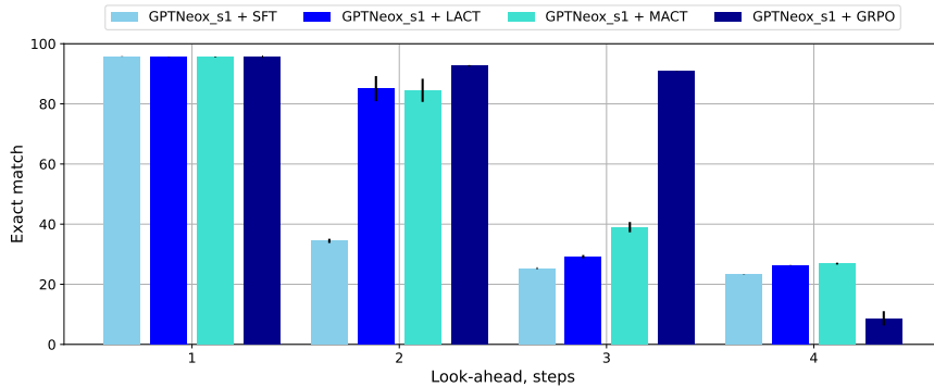
Figure 5: Without supervision on intermediate reasoning steps RL training with GRPO allows the model to extrapolate reasoning on 3 steps forward. While model and layer ACT variants extend it to 2 steps forward. However, 4 steps remains a challenging task for all approaches. All models are trained from GPTNeox checkpoint trained on 1 step forward prediction task.
