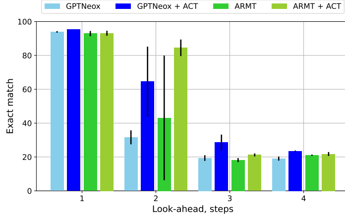
Figure 9: ACT outperforms the base model on multiple prediction horizons task. Exact match accuracy (mean \pm std) for cellular automata state prediction across different look-ahead horizons. Models receive initial 10 states followed by a special shift token (1-4) indicating prediction horizon.
