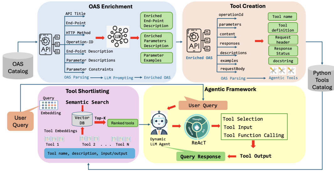
Figure 1: Automated Creation and Enrichment (ACE) Framework
