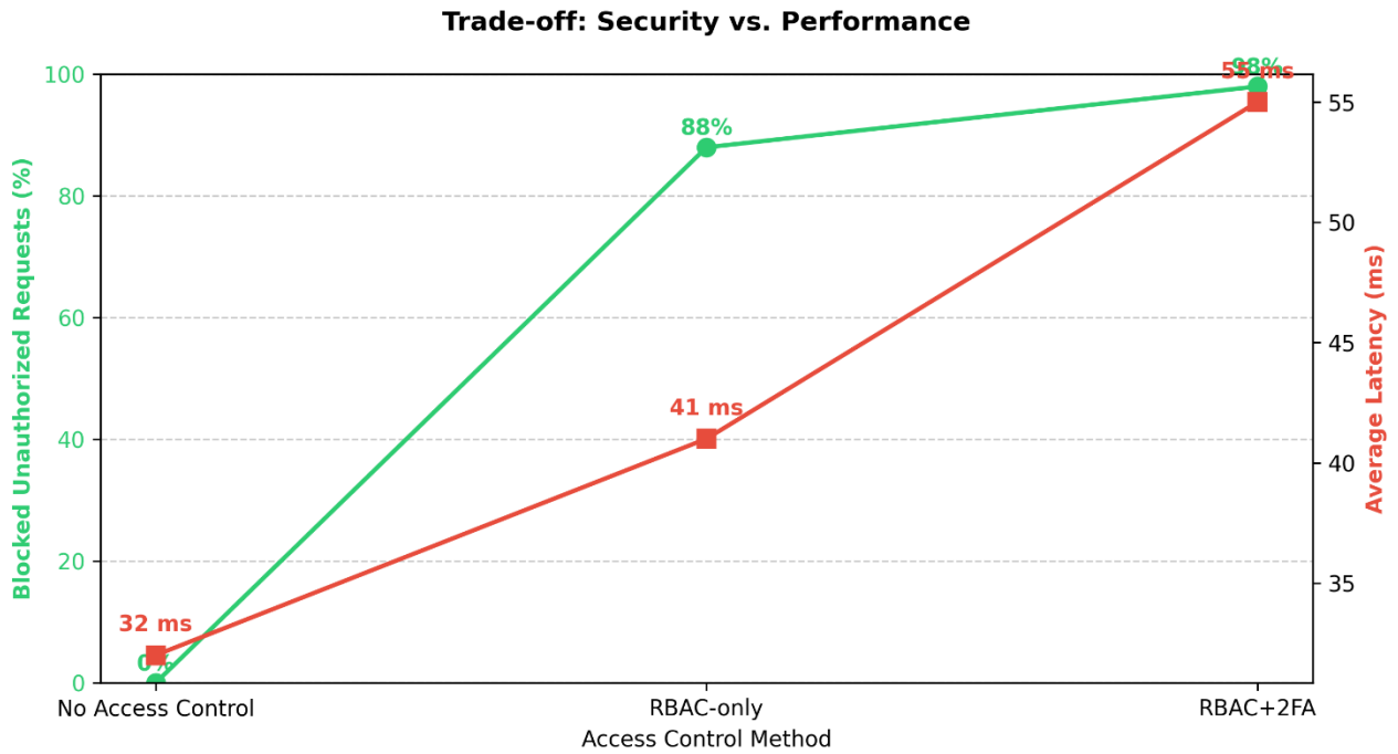
Figure 13. Security vs Performance
