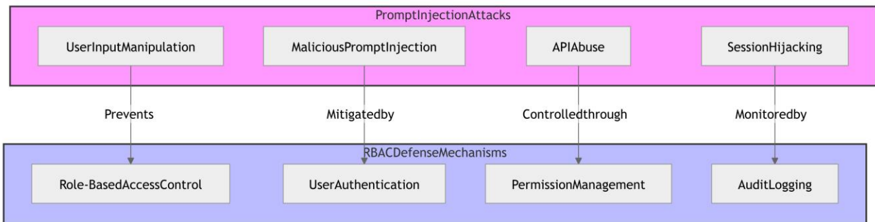
Figure 2: Prompt Injection Attack Vectors and RBAC Mitigation
