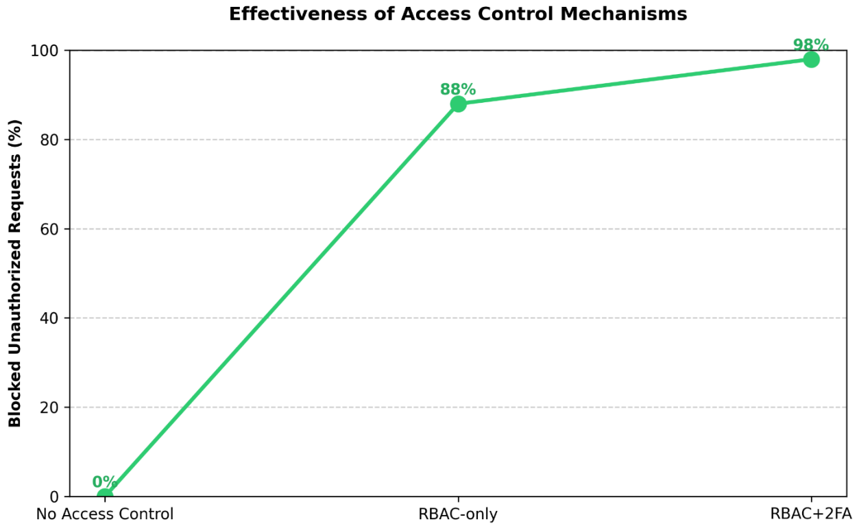
Figure 12. Effectiveness of Access Control Mechanisms
