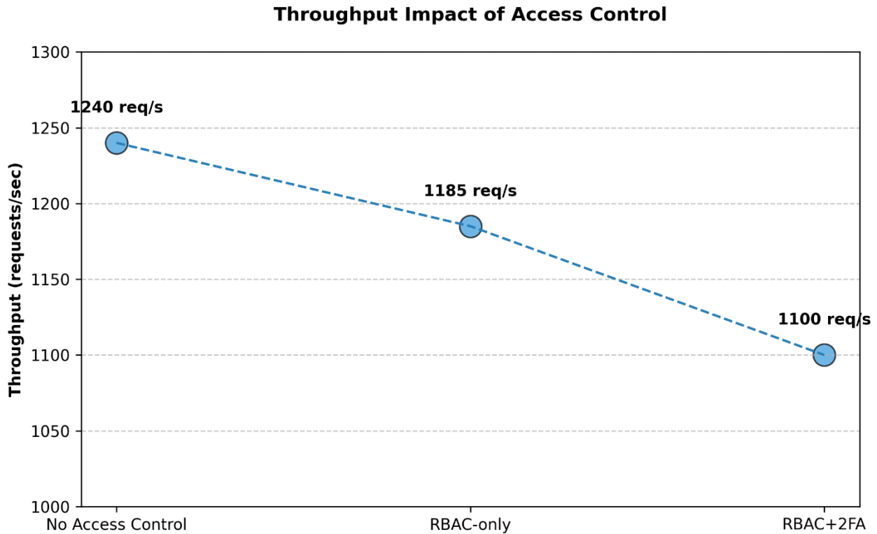
Figure 10. Throughput Impact of Access Control
