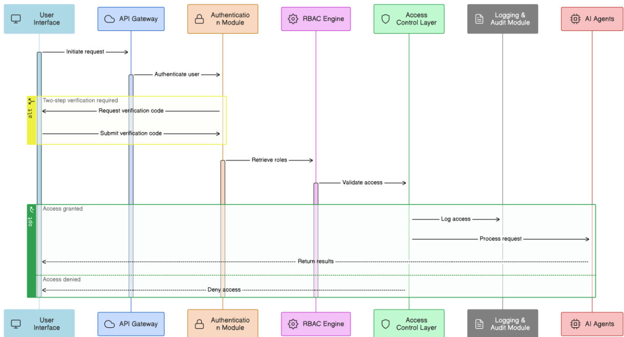
Figure 4: RBAC Framework Architecture in MYWAI
