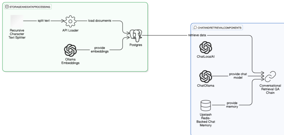
Figure 9: AI Agent Flowise Architecture
