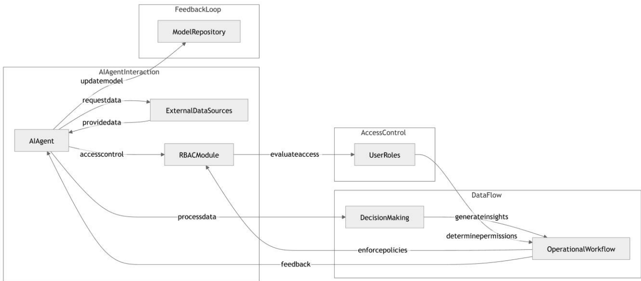
Figure 1: AI Agent System Architecture with RBAC Integration
