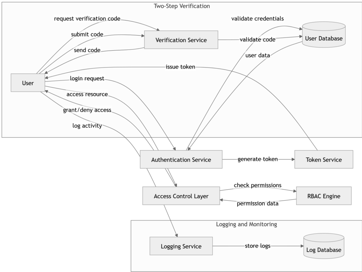
Figure 5: Access Control and Two-Step Authentication Flow
