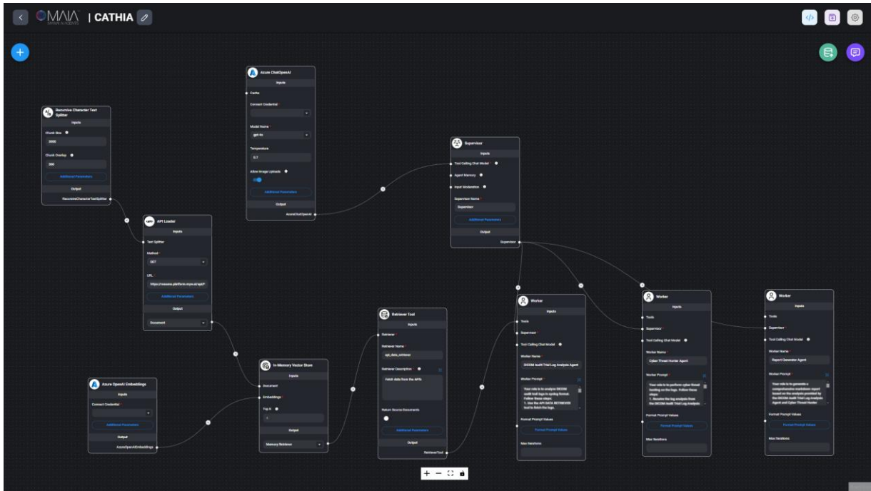
Figure 7: MultiAgent Flowise Retrieval Chain
