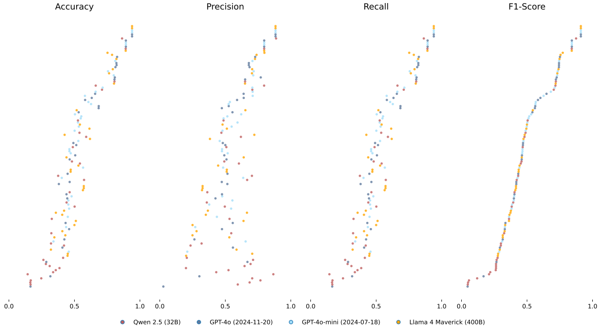
Figure 1: Goodness-of-Prediction Metrics of Synthetic Samples Against Ground-Truth Probabilistic Sample
