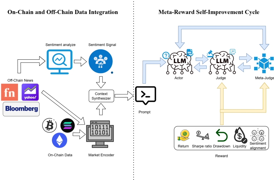
Figure 1: Overall Architecture of Meta-RL-Crypto. The system consists of a shared LLM that cyclically adopts the roles of Actor , Judge , and Meta-Judge . Market signals (on-chain metrics, off-chain news, sentiment scores) are encoded into structured prompts used by the Actor to generate forecasts. Each prediction is then scored by the Judge using a multi-dimensional reward vector, which the Meta-Judge uses to enforce preference consistency and evaluate the Judge itself.
