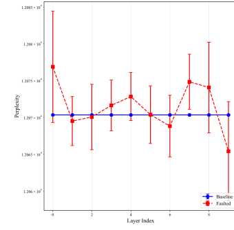
Fig. 2: Perplexity under Layerwise Bit-Flip Faults for GPT2 on Wikitext2
