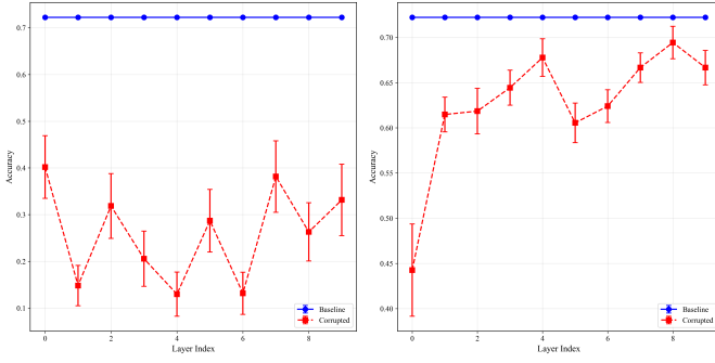
Fig. 1: DistilBERT on IMDB under Random Noise Injections with p = 0.1 (left) and p = 0.05 (right).
