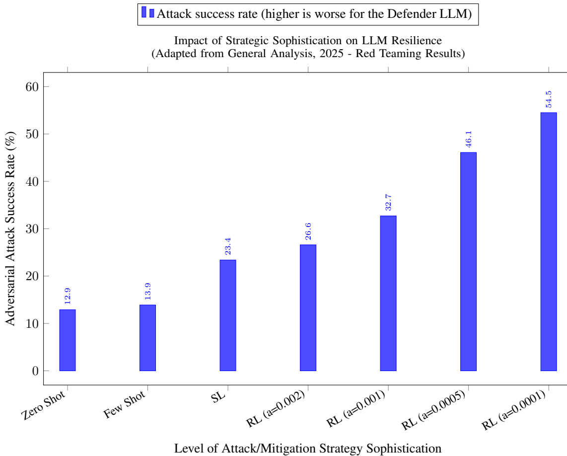
Figure 4: This graph illustrates how more sophisticated attack strategies (analogous to the lack of robust mitigation strategies or exploited vulnerabilities) achieve a higher success rate in inducing failures in a target LLM (GPT-4o). It demonstrates the need for equally sophisticated defense (mitigation) strategies. The X-axis represents different attack algorithms from the General Analysis study, interpreted here as levels of challenge or sophistication to which a legal RAG system must be resilient.
