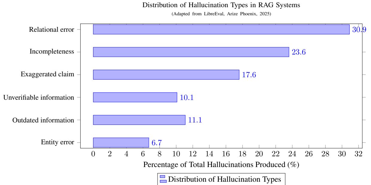
Figure 6: Percentage distribution of the different types of hallucinations actually produced in the responses of language models with RAG, according to the LibreEval1.0 dataset. This distribution highlights the most common challenges that mitigation strategies must address.
