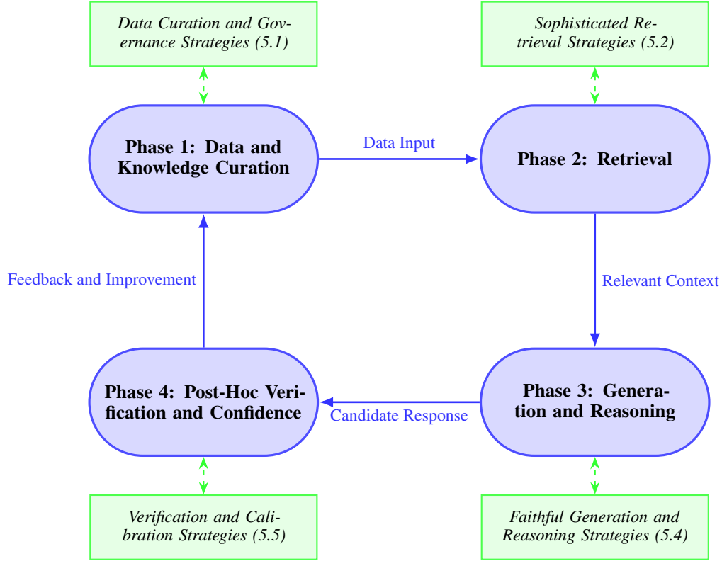
Figure 5: Cyclical model of a Legal RAG system and strategic intervention points for optimization and mitigation of hallucinations. The specific strategies (referenced by subsection of the essay) are applied at each phase to improve the overall reliability of the system.
