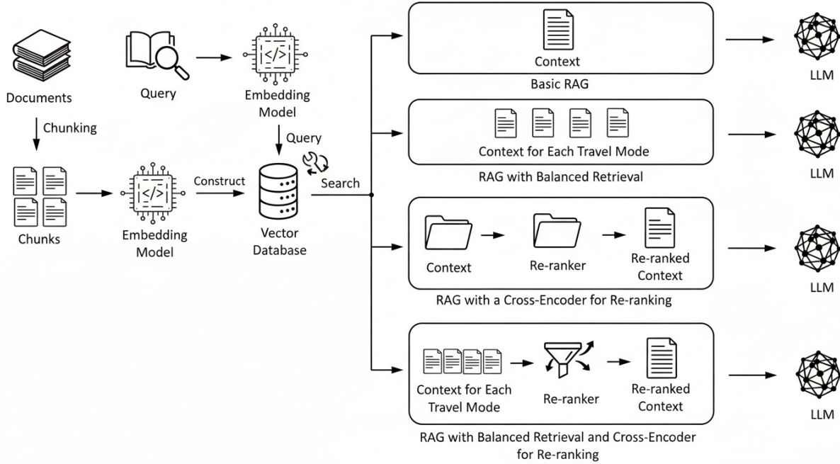
Figure 3: Schematic diagram of a retrieval-augmented generation (RAG) system. The flow illustrates how a user query (Input Query) is enriched with contextual information retrieved from an external knowledge base (Vectorstore) before being sent to the LLM. This process anchors the response in verifiable data, mitigating the generation of hallucinations. Adapted from Yiming Xu et al. (2025).
