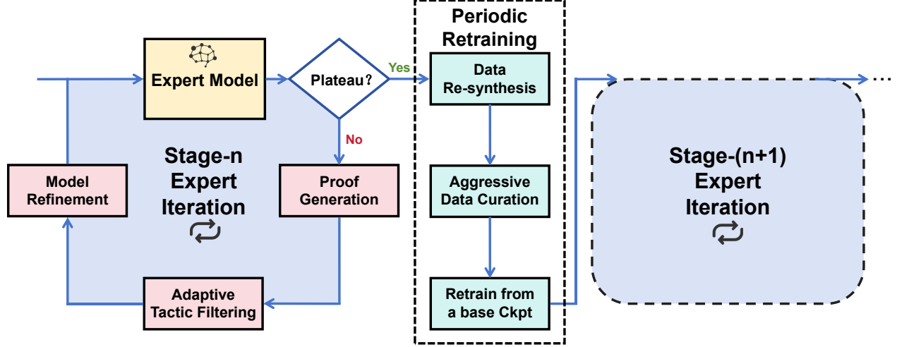
Figure 1 Overview of the training-time scaling up architecture. The process begins with a current expert model. The system then evaluates the model’s performance to check for a plateau, which determines the subsequent path. If performance is improving, the model enters an inner expert iteration loop that involves generating new proofs, applying Adaptive Tactic Filtering , and refining the model. Conversely, if performance has plateaued, the system triggers the outer retraining loop , which consists of Data Re-synthesis , Aggressive Data Curation , and retraining the model from a base checkpoint. Upon completion, this retraining loop yields a new, improved expert model, which then serves as the starting point for the next cycle of evaluation and iteration.
