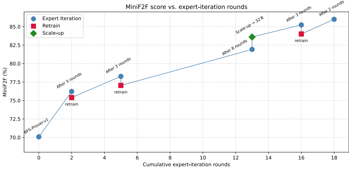
Figure 3 Sustained Performance Improvement through Expert Iteration and Periodic Retraining. This graph plots the prover’s performance on the MiniF2F benchmark against the number of expert iteration rounds. Performance steadily increases (blue circles) but eventually begins to plateau as the model settles into a local optimum. To counteract this, we periodically conduct a "soft reset" (red squares). This involves using the current expert model to re-solve all past problems to generate a cleaner, more efficient dataset, which is then used to retrain the model from a base checkpoint. This procedure allows the model to break out of its local optimum and continue improving, as evidenced by the significant performance jumps following each retraining phase. A model scale-up to 32 billion parameters is also shown (green diamond).
