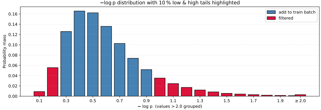
Figure 2 Tactic-Level Data Filtering Based on the Perplexity Distribution. This histogram shows the probability distribution of tactic perplexity (represented as negative log-probability) from a single round of expert iteration. We filter out the low- and high-perplexity tails, shown in red. The low-perplexity tail represents overly simple tactics the model is already confident in, while the high-perplexity tail often consists of noisy or unnecessarily complex tactics. By training only on the central part of the distribution (blue), we focus the model’s learning on challenging yet meaningful examples, which prevents overfitting and encourages a smoother, more stable improvement in reasoning capabilities.
