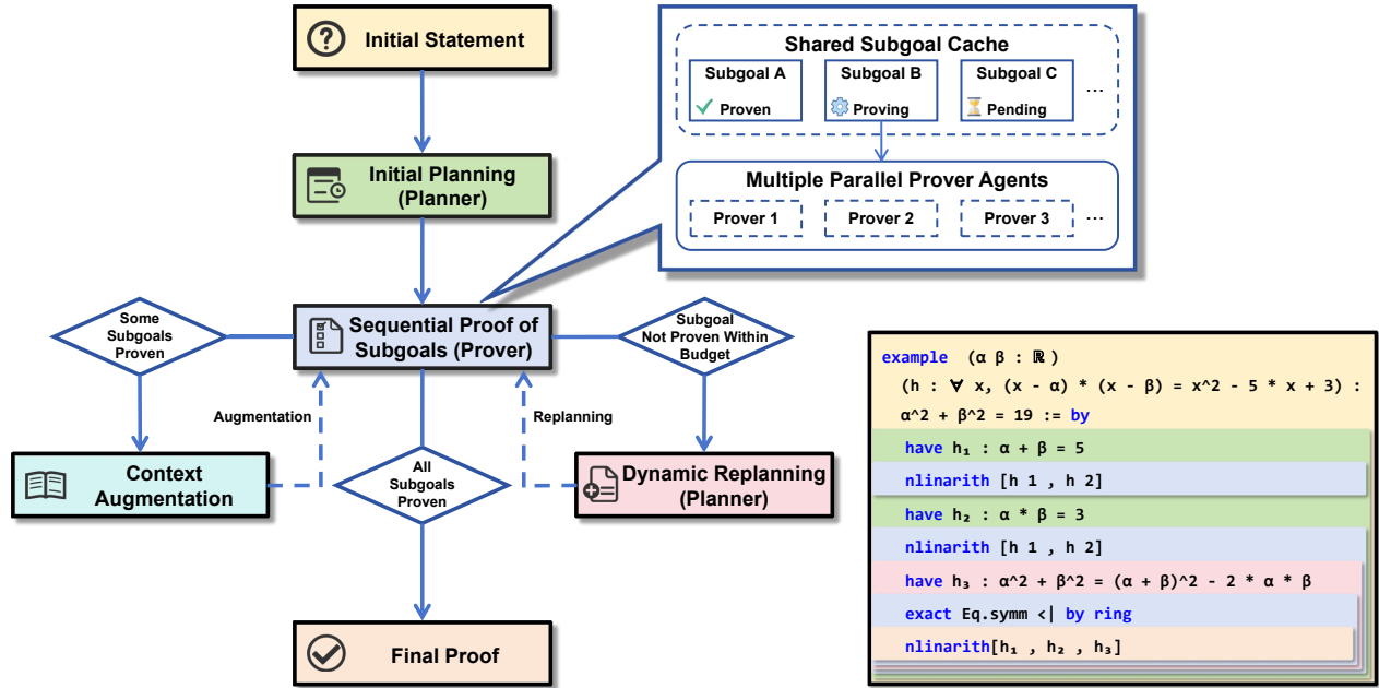
Figure 4 Overview of the planner-enhanced multi-agent tree search architecture. The Planner agent decomposes the main theorem into a sequence of simpler subgoals, which are managed in a Shared Subgoal Cache and solved in parallel by multiple Prover agents. Successfully proven subgoals augment the main proof’s context, while failures can trigger a Dynamic Replanning loop. The inset provides a toy example, demonstrating how proving intermediate lemmas ( h_1, h_2, h_3 ) facilitates the proof of the final goal.
