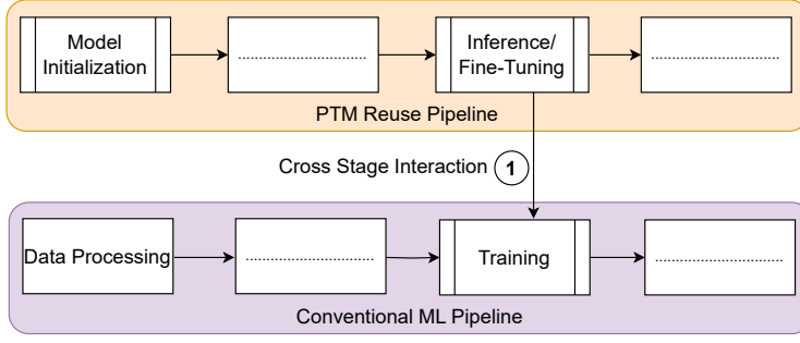
Fig. 10: Feedback Guidance: The PTM performs inference to produce outputs that are used to compute a loss, which is then passed ① to another pipeline and used during its training .
