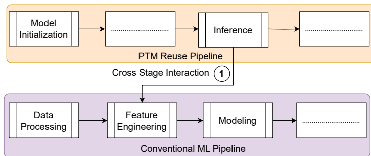
Fig. 9: Feature Handoff: The PTM generates outputs during inference and passes them (①) to the feature engineering stage of a downstream pipeline, enabling task-specific models to reuse pretrained representations.
