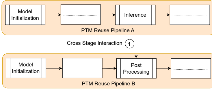
Fig. 12: Post-Processing Refinement. The PTM A performs inference to generate outputs that are used (①) to refine PTM B’s outputs during its postprocessing stage.
