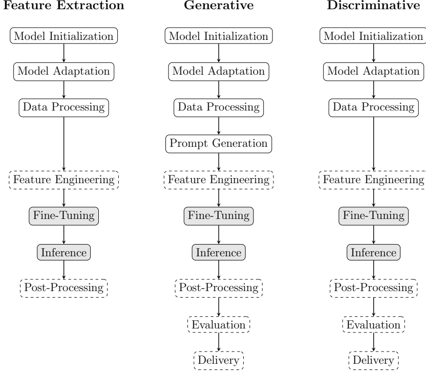
Fig. 8: Visualization of three pipeline organizations for reusing pretrained models. Grey boxes indicate stages common to most pipelines, i.e. , Fine-Tuning and Inference. Dashes indicate optional stages.
