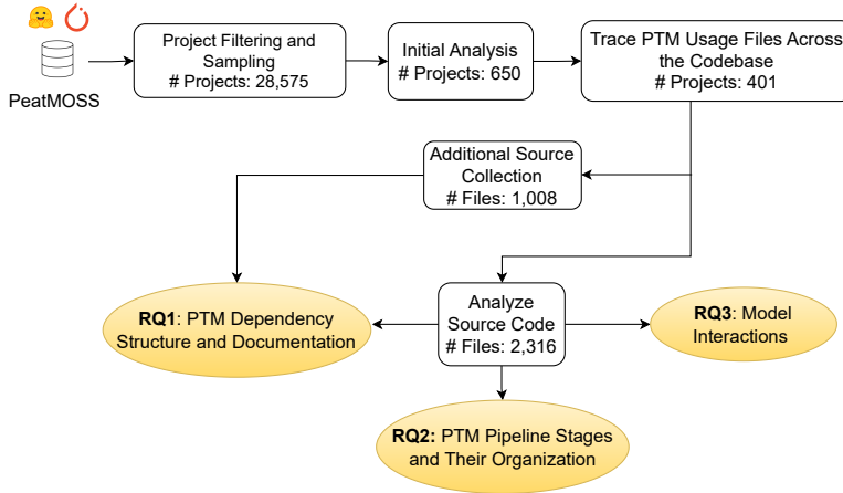
Fig. 4: Study Overview: Projects were filtered and analyzed to investigate PTM usage, pipeline stages, and model interactions.
