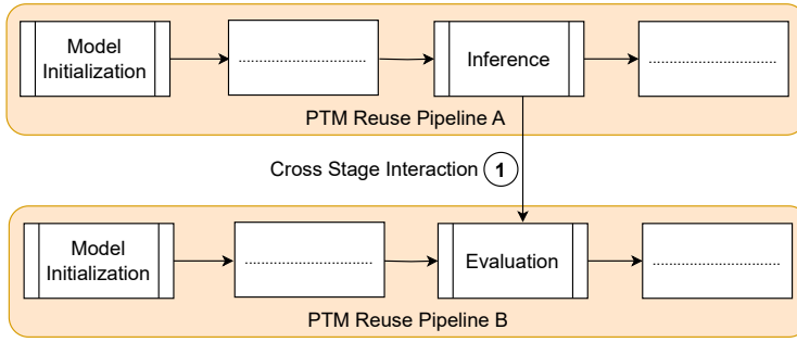
Fig. 11: Post-Processing Refinement: The PTM A performs inference to generate outputs that are used (①) to evaluate PTM B’s outputs during its evaluation stage.
