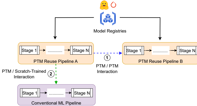
Fig. 2: Overview of PTM reuse pipelines and their interactions within a project. PTM Reuse Pipeline A reuses models from registries such as Hugging Face and PyTorch. It may interact with other pipelines in two ways: PTM/PTM Interaction (①): interaction with PTM Reuse Pipeline B. PTM/Scratch-Trained Interaction (②): interaction with Conventional ML Pipeline. Dashed arrows indicate optional steps. Ellipses show omitted intermediate stages.
